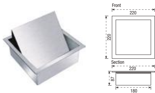
Dustbin Cover Counter Mounted
