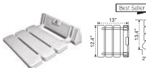
Chair/Stool Foldable (Wall Mounted)
