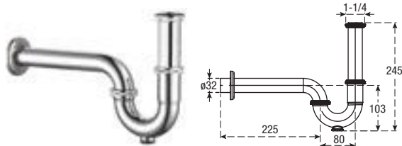
P Trap
