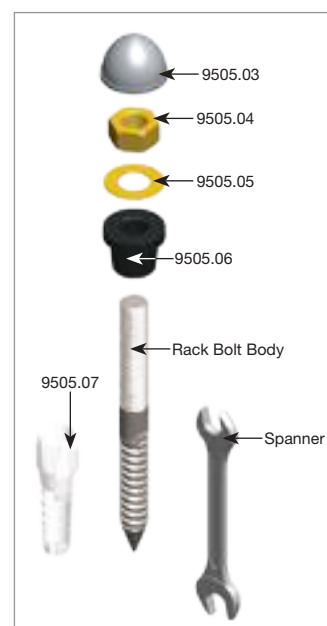
Breakup view of 9505 parts
