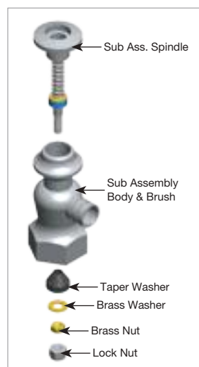
Breakup view of 11851 parts
