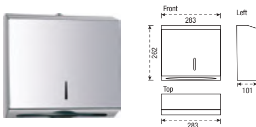
Dispenser for Paper Towel
