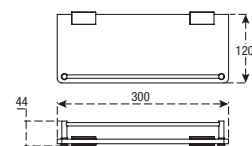
Glass Shelf with Rail-Rectangular (Wall Brackets)
