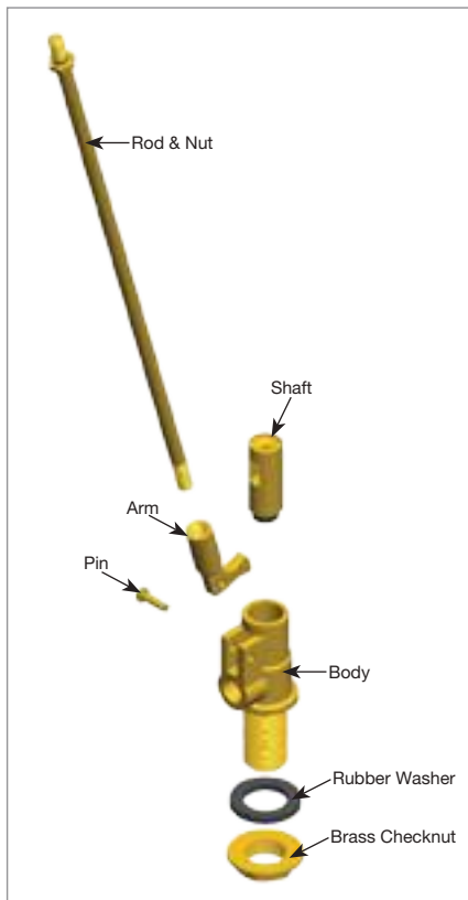
Breakup view of 14101 parts
