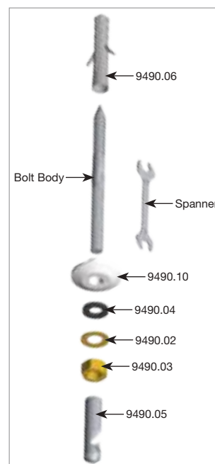
Breakup view of 9490 parts
