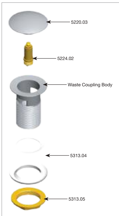
Breakup view of 5220 Parts
