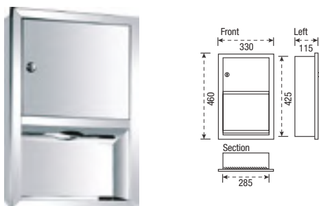
Dispenser in Box for Paper Towel
