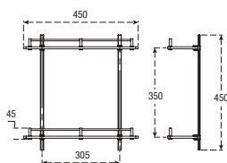
Double Shelf-Rectangular
