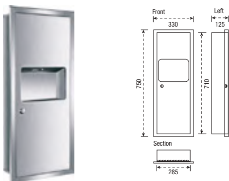
Dispenser and Dustbin for Paper Towel
