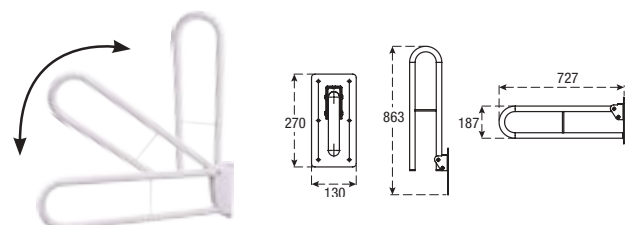
Grab Bar for Handicapped Persons
