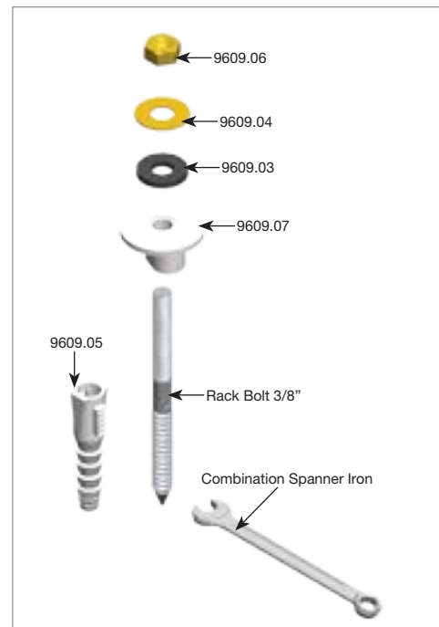
Breakup view of 9609 parts
