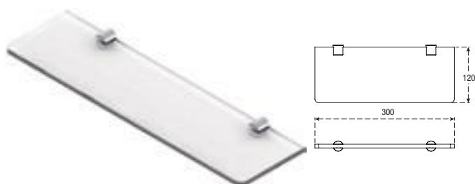
Glass Shelf without Rail-Geometrical (Wall Brackets)
