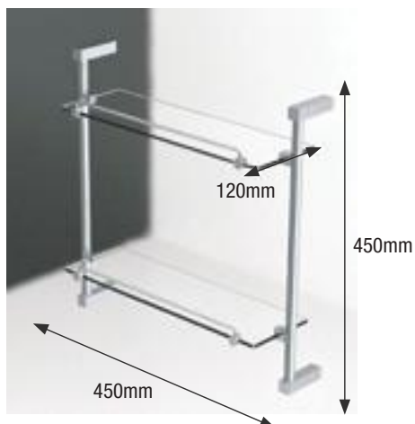
Double Glass Shelf-Square
