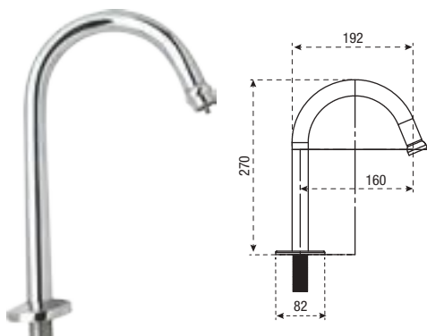
Pillar Cock Touch On OFF for Counter Top Basins (Fits all counter top basins)
