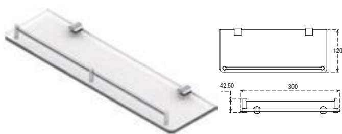
Glass Shelf with Rail-H 2 O
