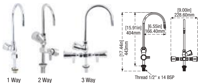
Lab Cock Extended Spout
