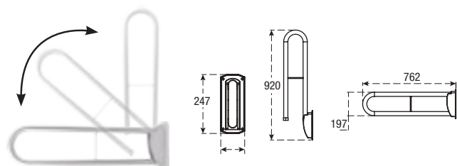
Grab Bar for Handicapped Persons
